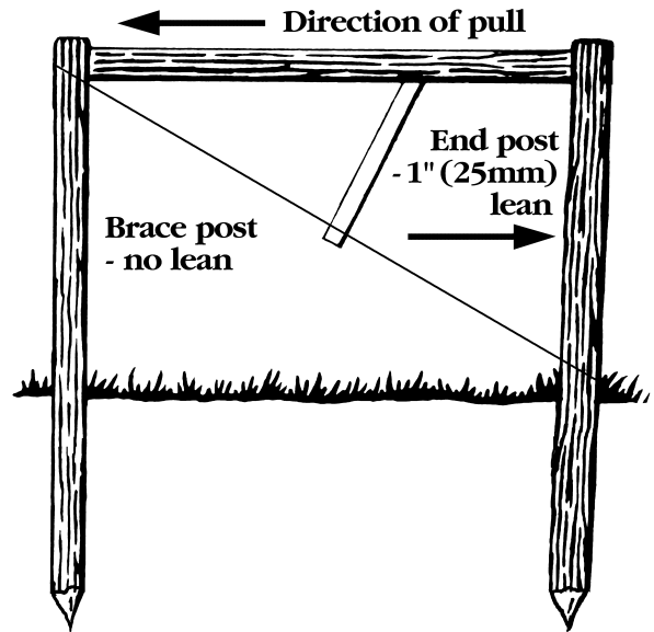
FIGURE 2. Single-Span Brace Assembly
