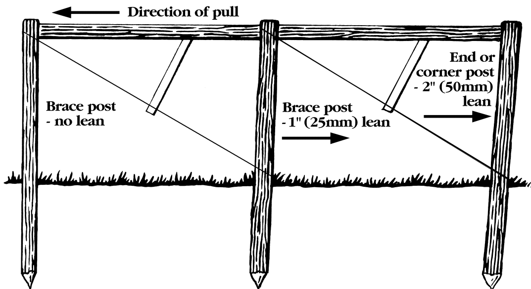
FIGURE 3. Double-Span Brace Assembly
